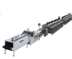
20-Station Large Format POS Kitting into Wrapper
